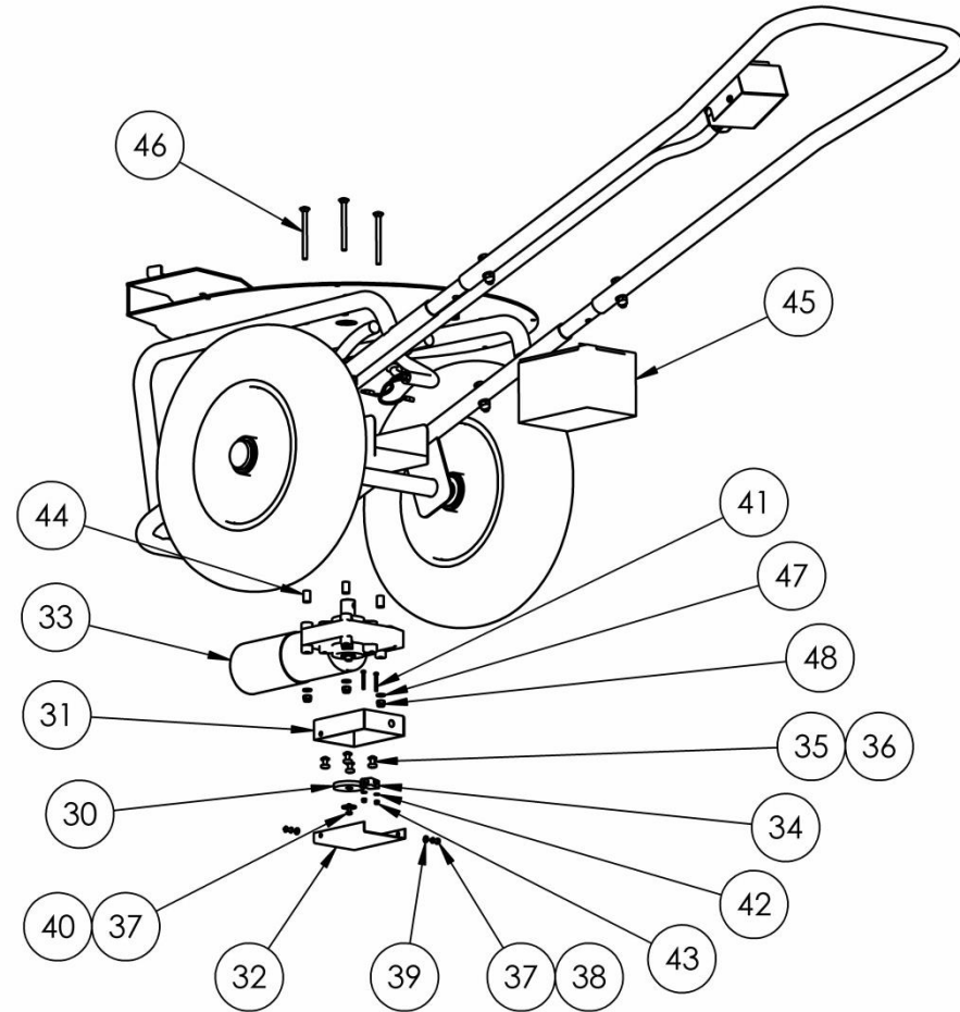
MOTOR COMPONENTS & BATTERY
