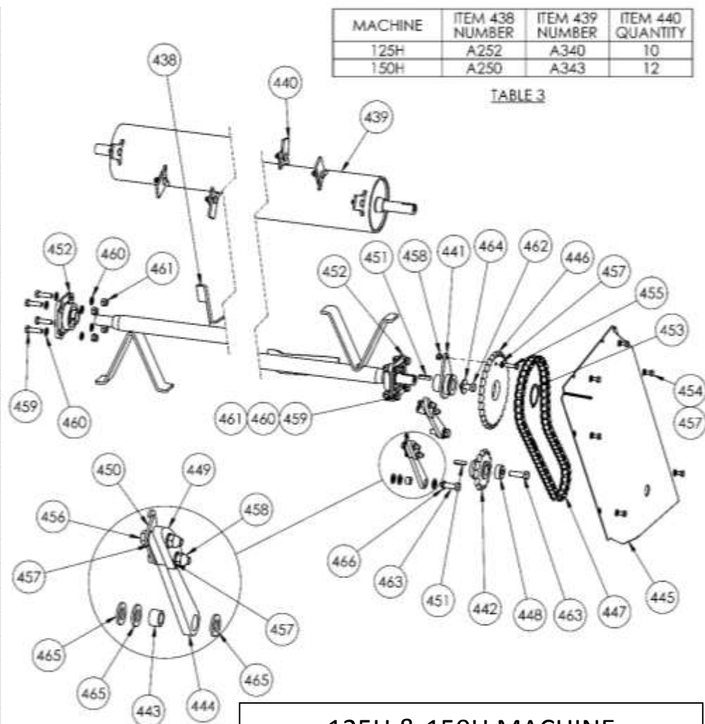
125H & 150H MACHINE TOP AGITATOR COMPONENTS
